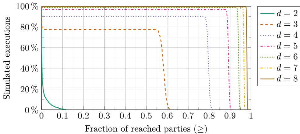
Figure 3: Results for simulations of \text{FFlood}(d) for different values of d and a fixed n = 8192 . The graphs show the percentages of the simulated executions (on the y-axis) where at least a certain fraction of parties received the message (on the x-axis).
