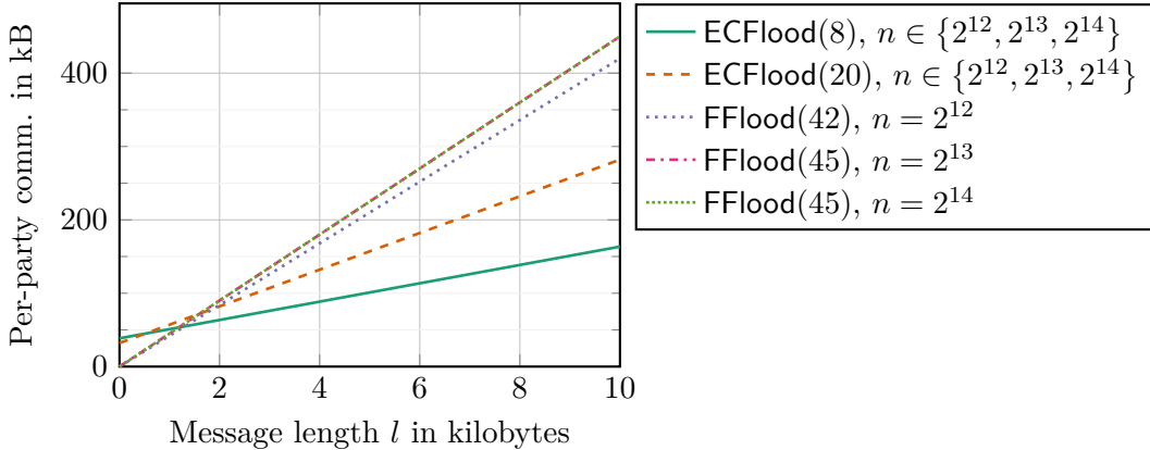
Figure 10: Per-party communication as a function of the message length l in kilobytes with parameters chosen such that all parties receives the message for all 100 000 simulations. For ECFlood(8), \mu = 25 shares is used and the reconstruction threshold for the erasure codes is \mu - \rho = 16 . For ECFlood(20), \mu = 10 shares is used and the reconstruction threshold for the erasure codes is \mu - \rho = 8 .
